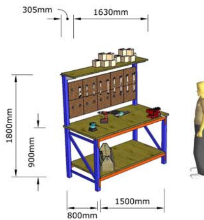
Standing Workbench with Top Level Storage Option 2
