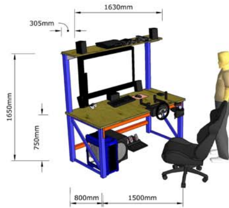
Seated Workbench with Top Level Storage Option 2
