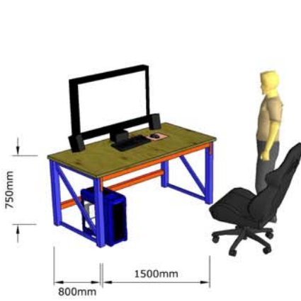
Seated Workbench Option 1
